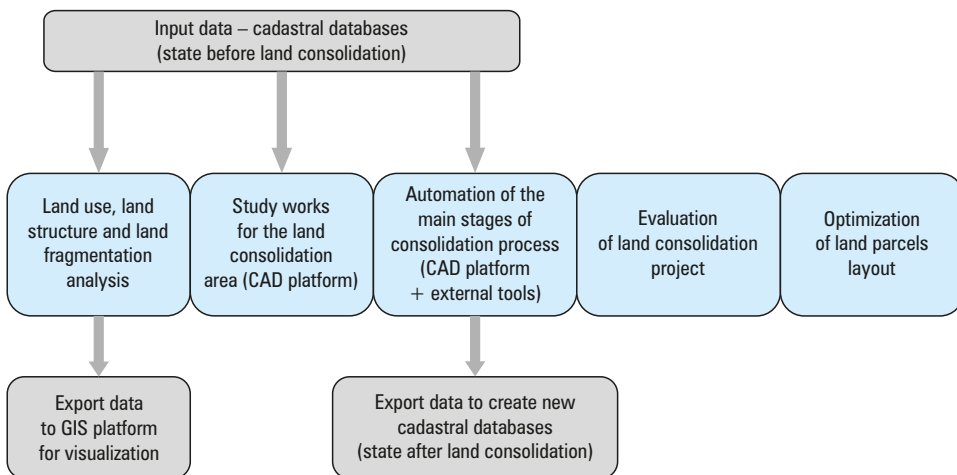
Fig. 2. Structural chart of MKSCAL system
