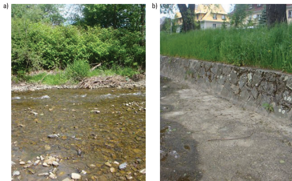
Fig. 1. Fragments W_{1/1} and W_{1/2} , a) Wieprzówka thread, b) riverbed with concrete bottom and concrete bank reinforcements
